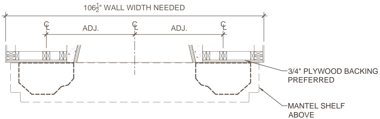
3 FRAMING PLAN SCALE: 1/2"=1'-0"
