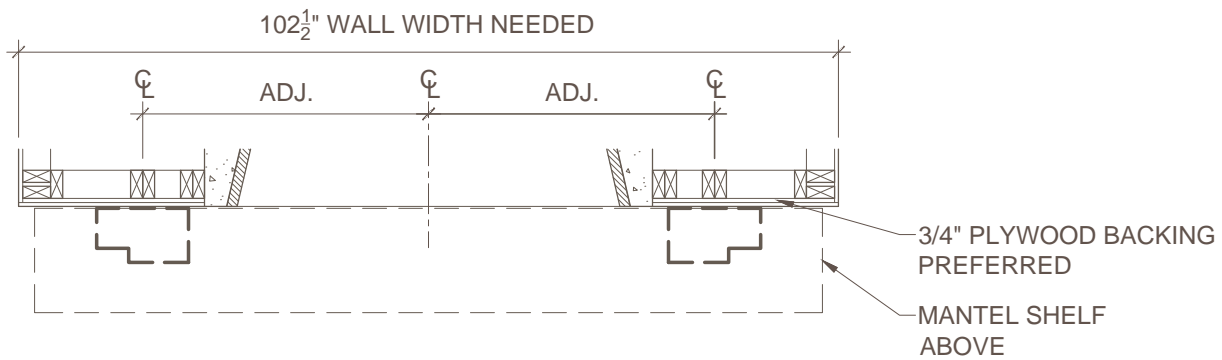
3 FRAMING PLAN SCALE: 1/2" = 1'-0"
