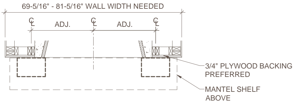
3 FRAMING PLAN SCALE: 1/2"=1'-0"
