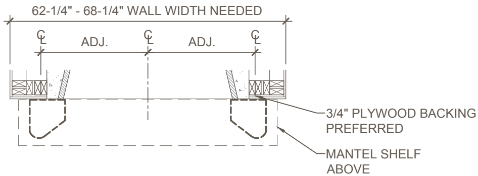
3 FRAMING PLAN SCALE: 1/2"=1'-0"
